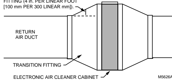
Fig. 3. Change duct size gradually to minimize turbulence.
